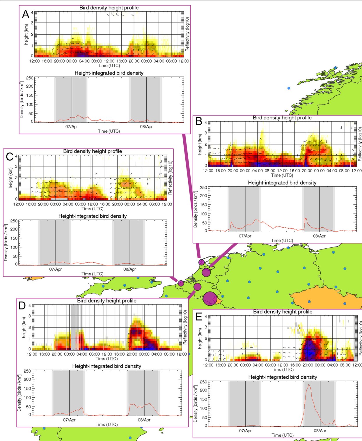
Figure 2 Mass bird migration observed on five operational weather radars. Nocturnal bird migration measured by two operational weather radars in the Netherlands ( A . Den Helder and B . De Bilt) and three operational weather radars in Belgium ( C . Jabbeke, D . Zaventem and E . Wideumont) on 7 and 8 April 2013 (for locations see purple circles on map, blue circles indicate other weather radars in the vicinity). The size of the purple circles represent the height-integrated bird density (birds/km 2 ) on 8 April 2013 at peak migration. Colours in upper graphs of each subplot indicate bird density (number of birds/km 3 ) with the wind bars indicating the birds' ground speed and flight direction, lower graphs in each subplot indicate the height-integrated bird density (birds/km 2 ), grey areas in these graphs indicate periods between dusk and dawn.
